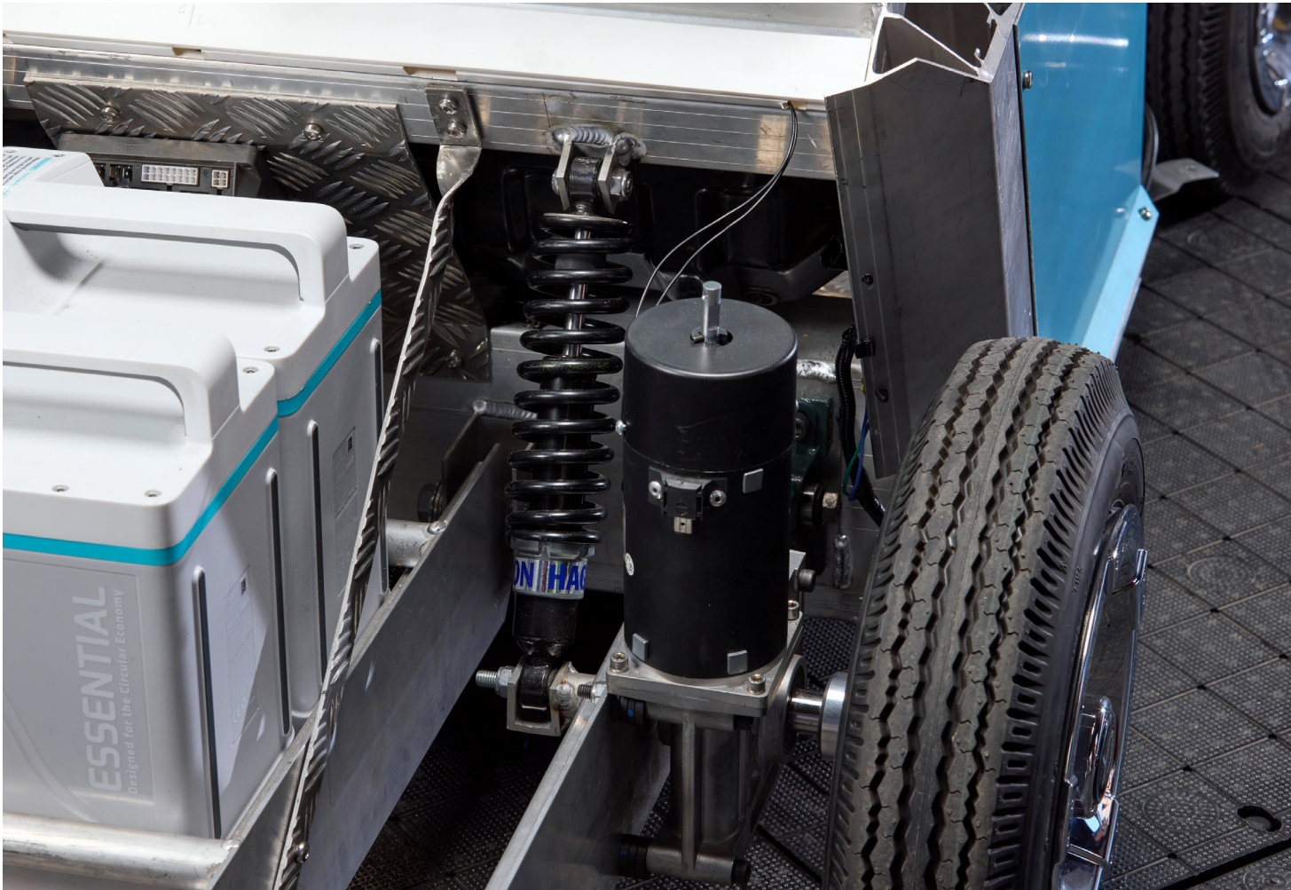
A Parvalux drive unit between the suspension and the wheel.
