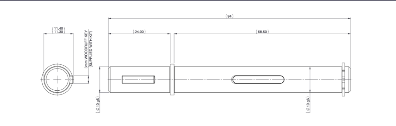
GB80 shaft extension kit
