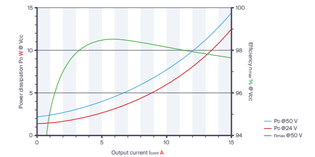
Power dissipation and efficiency
