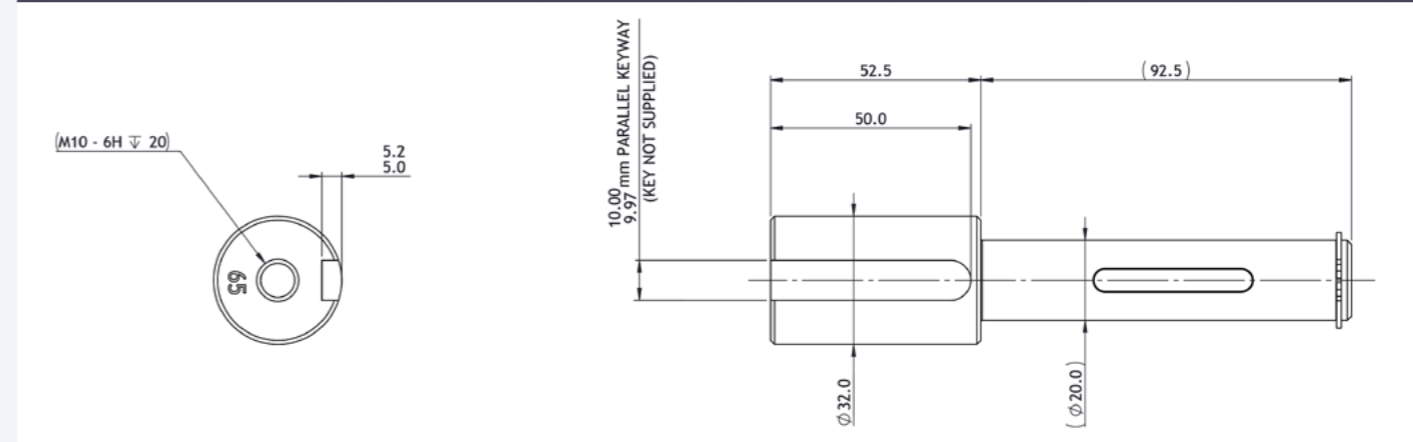
GB65 shaft extension kit 854742
