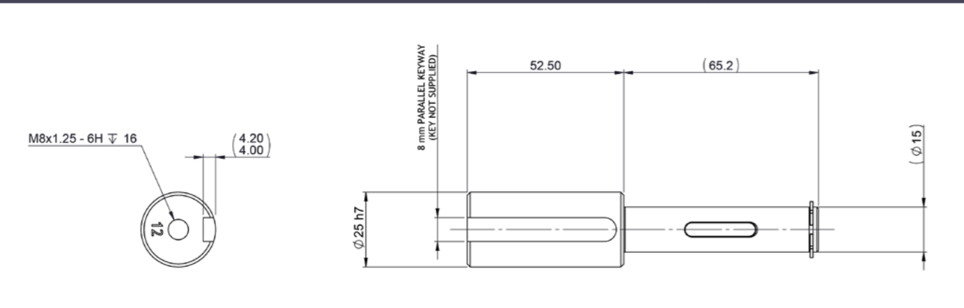
GB12 shaft extension kit 735903
