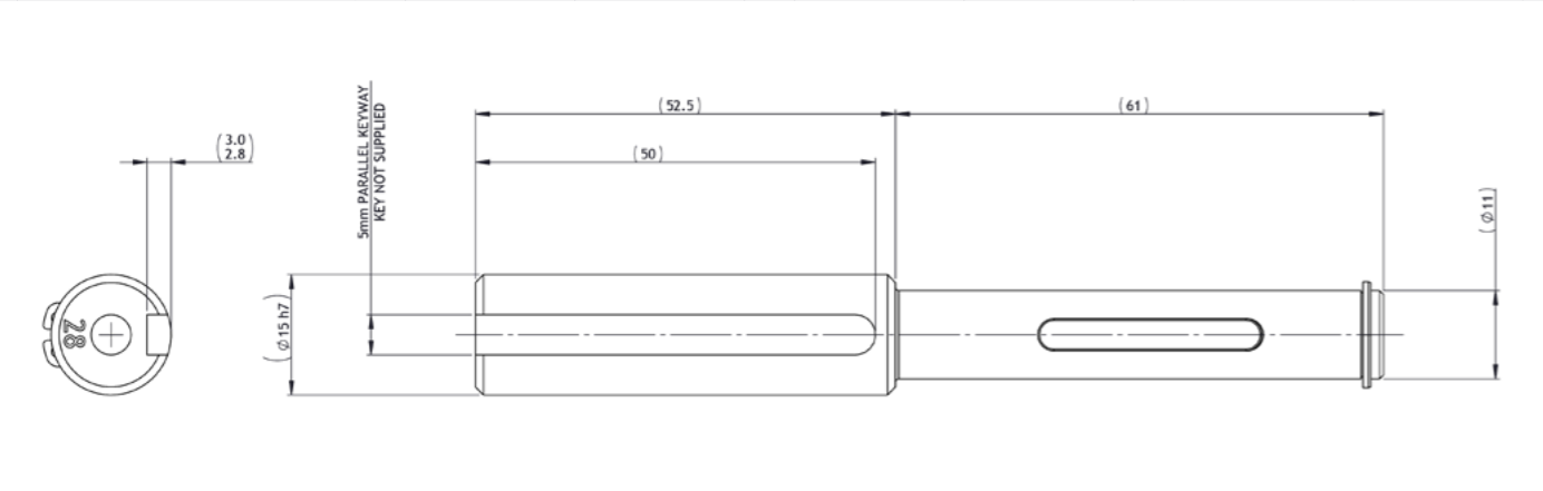
GB28 shaft extension kit 735908
