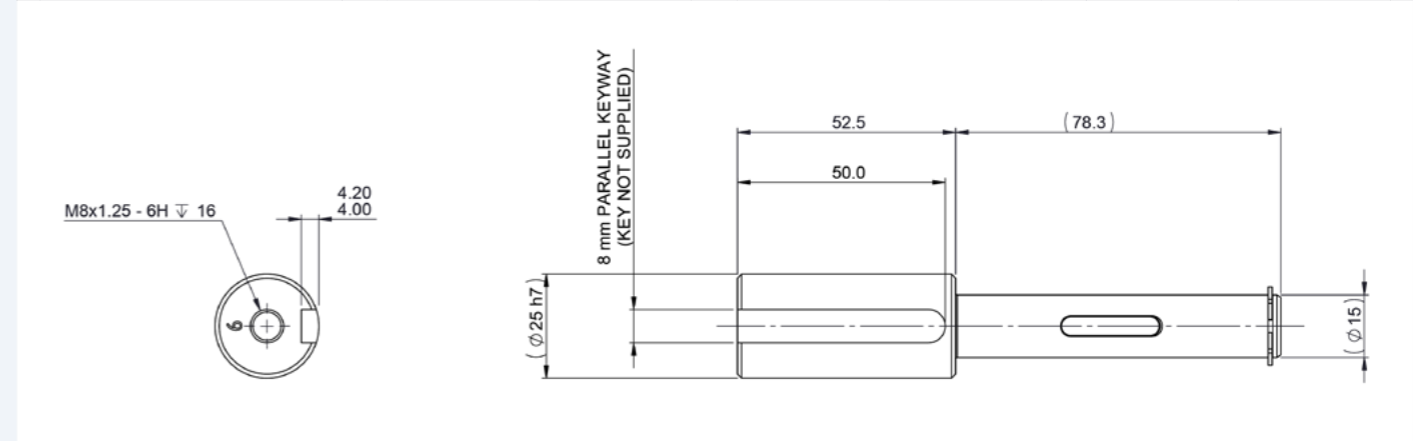
GB9 shaft extension kit 735898
